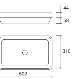
new product Semi inset basins MAEL Solid surface Bicolour without bottle trap or clicker waste 502 x 44 x 310 mm 97655 325 €
