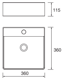
new product Countertop basin TALEA Matt white solid surface without bottle trap or clicker waste 360 x 115 x 360 mm 97649 305 €
