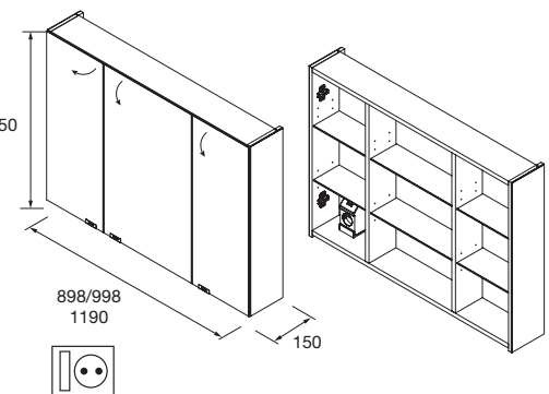
Cabinet ALLIANCE 900 3 soft close double mirror doors with switch and plug 898 x 650 x 150 mm 24592 648 € Cabinet ALLIANCE 1000 3 soft close double mirror doors with switch and plug 998 x 650 x 150 mm 23665 677 € Cabinet ALLIANCE 1200 3 soft close double mirror doors with switch and plug 1190 x 650 x 150 mm 24593 764 €
