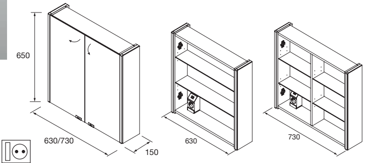
Cabinet ALLIANCE 700 2 soft close double mirror doors with switch and plug and LED side light, IP44 (21,5W) 730 x 650 x 150 mm 83154 686 €
