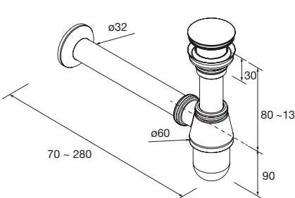
Open bottle trap valve with waste Chrome brass 16994 75 €
