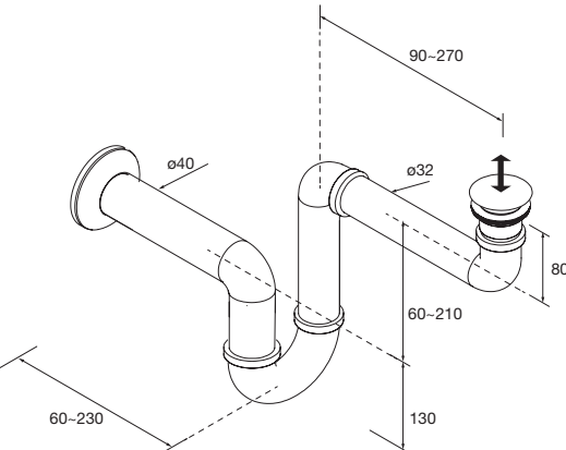
Reduced bottle trap plus clicker valve set 19366 68 €
