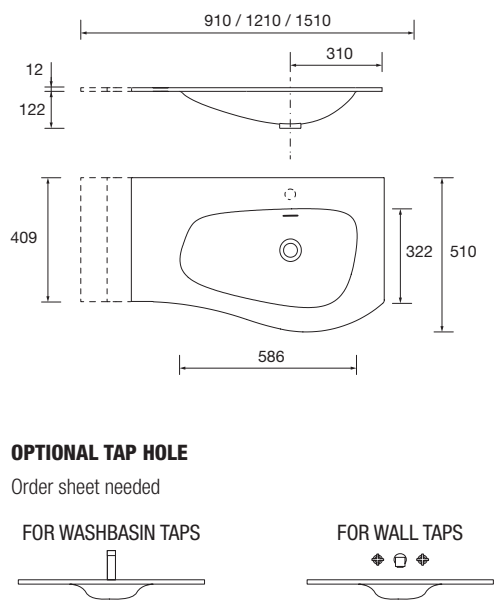
Basin MAM 1500 storage unit on the left Matt white solid surface without bottle trap or clicker waste 1510 x 12 x 510 mm 91123 667 €
