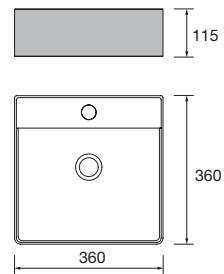
new product Countertop basin TALEA Solid surface Bicolour without bottle trap or clicker waste 360 x 115 x 360 mm 97652 325 €
