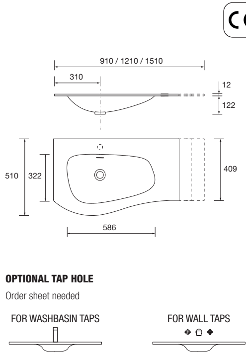
Basin MAM 1500 storage unit on the right Matt white solid surface without bottle trap or clicker waste 1510 x 12 x 510 mm 91122 667 €
