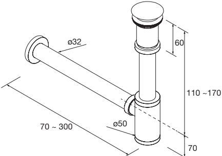
Bottle trap SMART with open valve 23032 95 €
