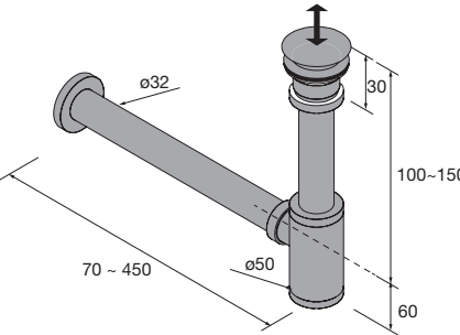
Bottle trap VINCI Matt black with clicker waste 26985 112 €
