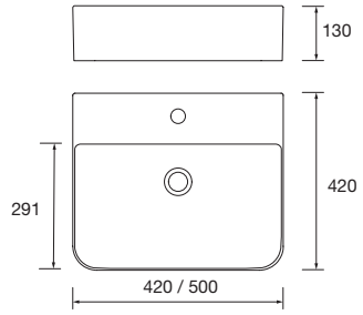
Countertop basin TENTO 500 White porcelain without bottle trap or waste 500 x 420 x 130 mm 24552 186 €
