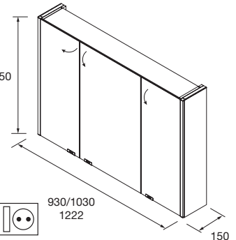
Cabinet ALLIANCE 1200 3 soft close double mirror doors with switch and plug and LED side light, IP44 (21,5W) 1222 x 650 x 150 mm 83166 999 €
