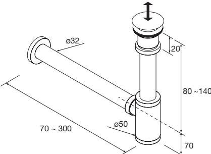
Bottle trap SMART Chrome with clicker waste 23033 101 €
