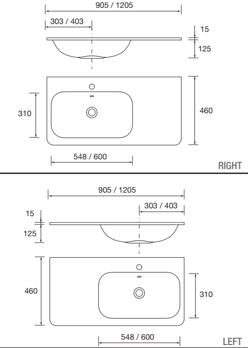
Basin UNIQ 1205 storage unit on the left Matt mineralsolid without bottle trap or clicker waste 1205 x 15 x 460 mm 24546 475 €
