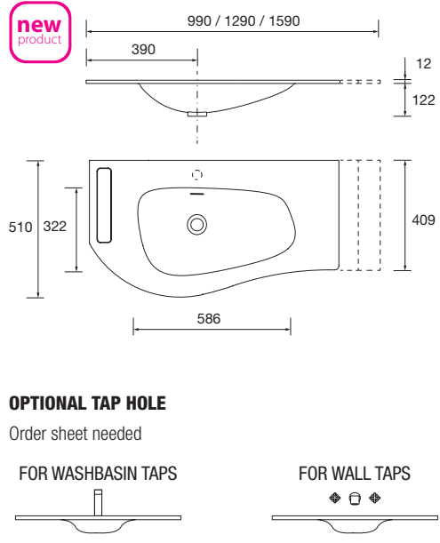
Basin MAM 1590 right with towel rail Matt white solid surface with towel rail, without bottle trap or clicker waste 1590 x 12 x 510 mm 97397 757 €
