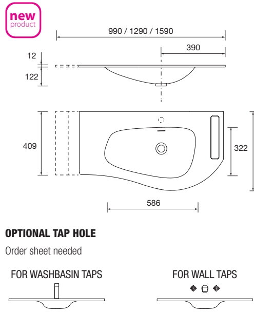
Basin MAM 1590 left with towel rail Matt white solid surface with towel rail, without bottle trap or clicker waste 1590 x 12 x 510 mm 97400 757 €
