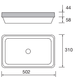
new product Semi inset basins MAEL Solid surface Bicolour without bottle trap or clicker waste 502 x 44 x 310 mm 97655 325 €
