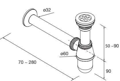
Drain pipe clicker Chrome brass 9699 63 €
