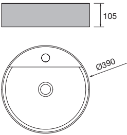
new product Countertop basin BICA Solid surface Bicolour without bottle trap or clicker waste Ø 390 x 105 mm 97648 325 €
