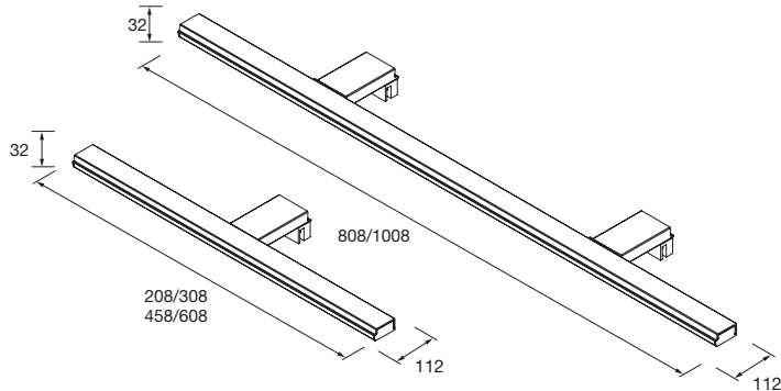
Light PANDORA 208 gloss chrome LED light (5 W- 5700°K) IP 44 multihook fastening 208 x 112 x 32 mm 24548 55 € Light PANDORA 308 gloss chrome LED light (8 W- 5700°K) IP 44 multihook fastening 308 x 112 x 32 mm 21735 67 € Light PANDORA 458 gloss chrome LED light (1x10 W- 5700°K) IP 44 multihook fastening 458 x 112 x 32 mm 23534 84 € Light PANDORA 608 gloss chrome LED light (1 x 11 W- 5700°K) IP 44 multihook fastening 608 x 112 x 32 mm 23535 107 € Light PANDORA 800 gloss chrome LED light (11 x 15 W -5700°K) IP 44 multihook fastening 808 x 112 x 32 mm 23536 143 € Light PANDORA 1008 gloss chrome LED light (1 x 15 W -5700°K) IP 44 multihook fastening 1008 x 112 x 32 mm 24549 170 €
